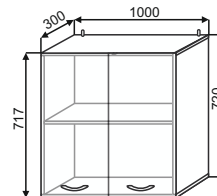
ШВ 1000 1000x720x300
