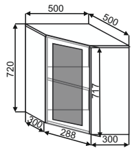
ВУС 500X500 500x720x500
