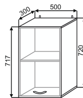
ШВ 500 500x720x300
