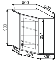
ШВУС(2) 500x500 500x900x500
