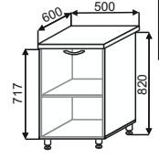
ШН 500 500x850x600
