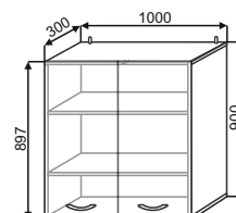
ШВ(2) 1000 1000x900x300
