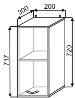
ШВ 200 200x720x300
