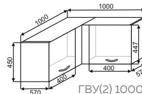
ГВУ(2) 1000 1000x450x570
